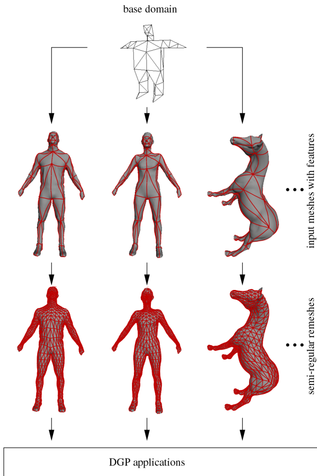
Figure 2: Multiple models are parameterized with respect to the same base domain using feature point (and edge) mappings. Subsequent remeshes ensure consistent sampling patterns for downstream DGP applications.
